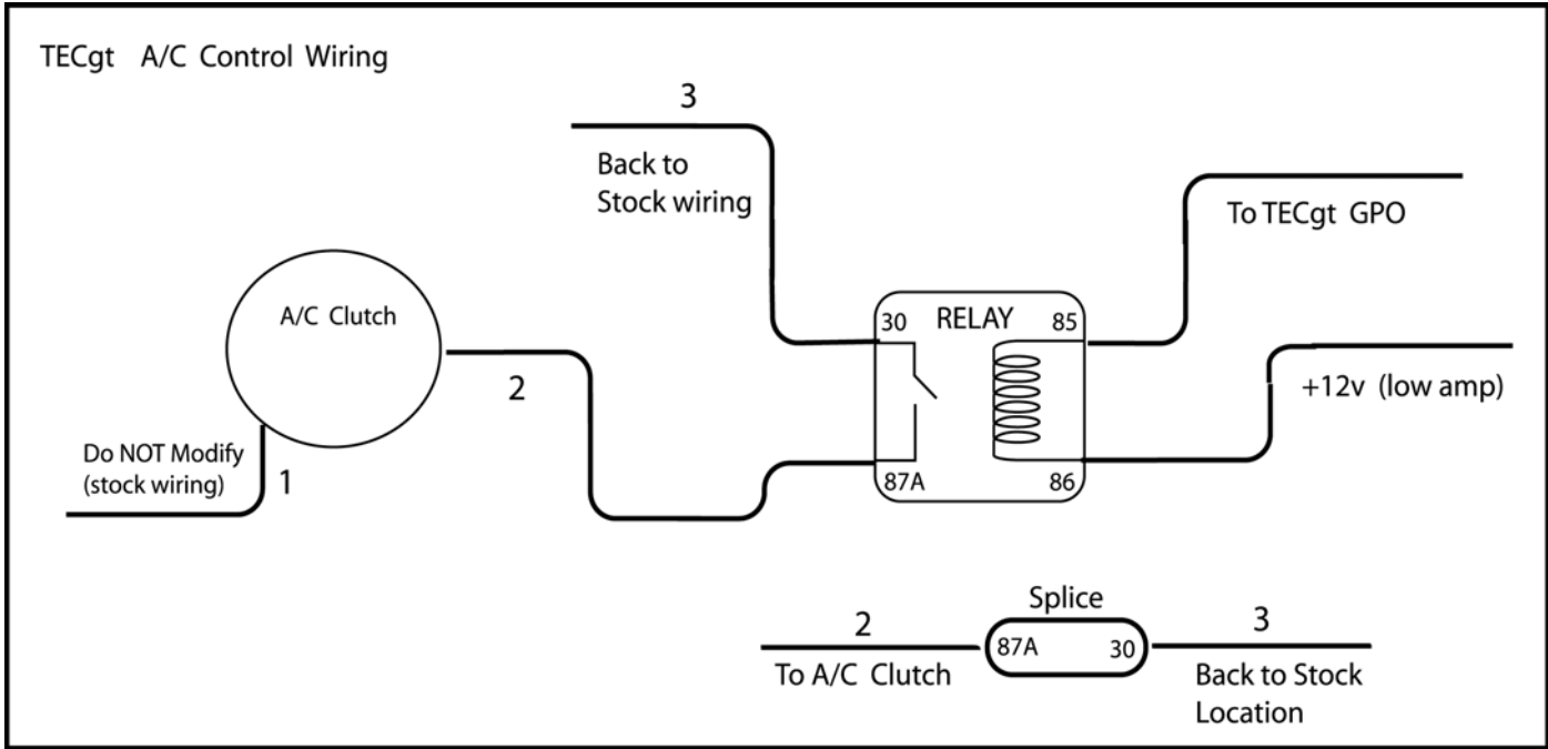
Figure H.2.3: Air conditioner control wiring. Note that the relay simply splices into either of the two wires on the A/C clutch with terminals 30 and 87a. When activated, the A/C control will break the (normally-closed) connection between 30 and 87a by grounding pin 85.
