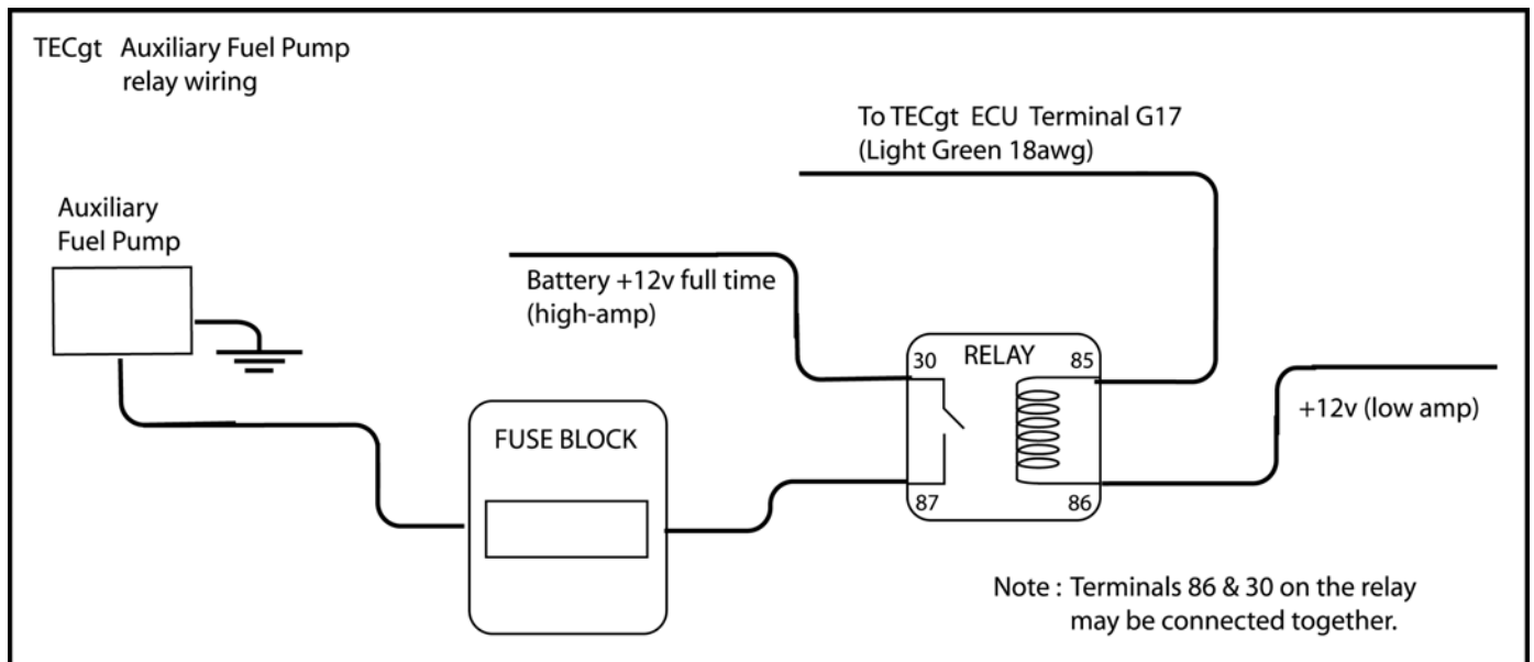
Figure H.2.4: Auxiliary fuel pump wiring.
