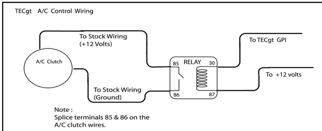
Fig. H.1.2: Air conditioner idle speed increase wiring.
