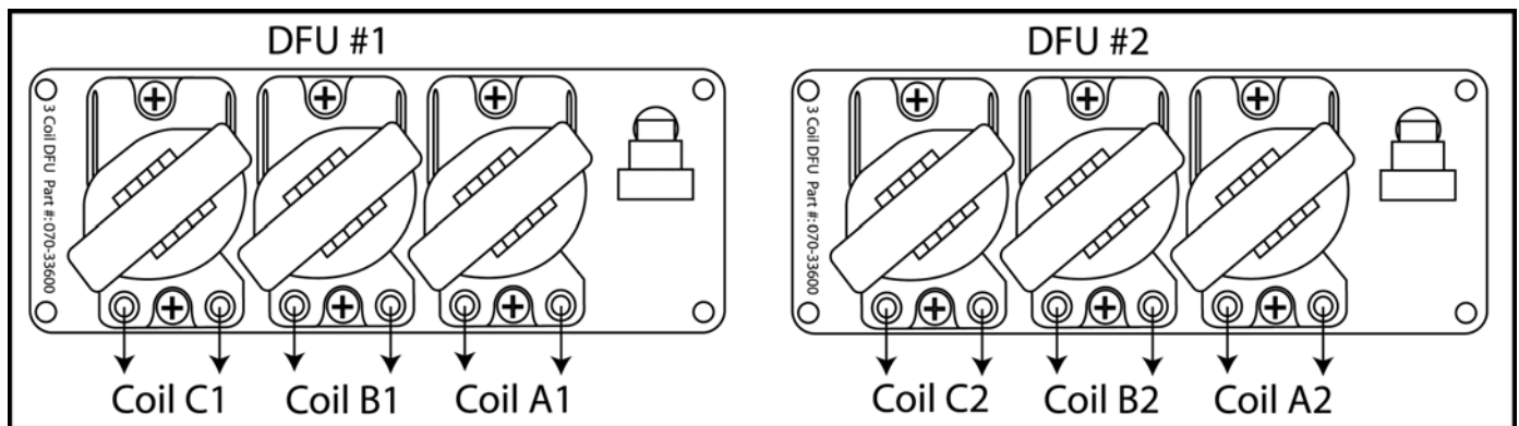
Figure C.2.1 : Coil notation
