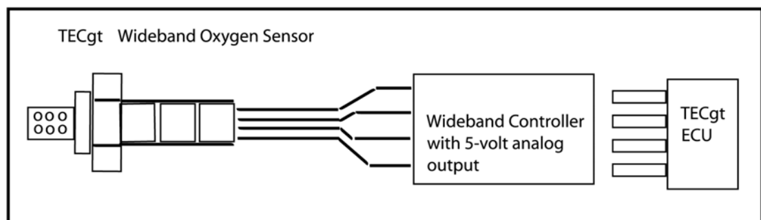
Figure G.6.1 - Typical Wideband Configuration
