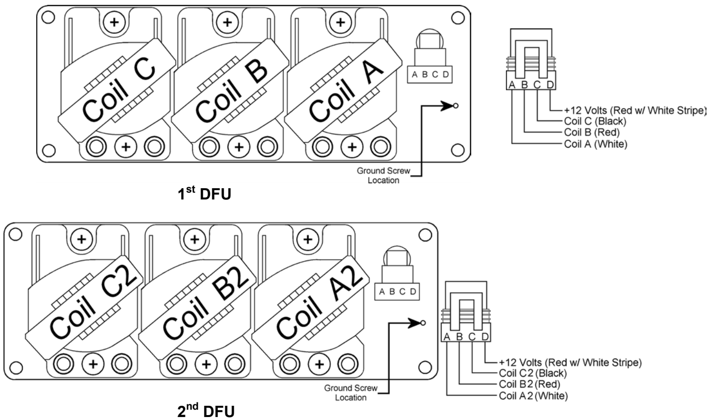
Figure C.2. 5: (The above picture from a twin-plug 6 Cyl. is for reference only), this application does not pertain to the TECglt , if running a V8 the first DFU will have coils A1, B1 the second DFU will have coils A2, B2.
