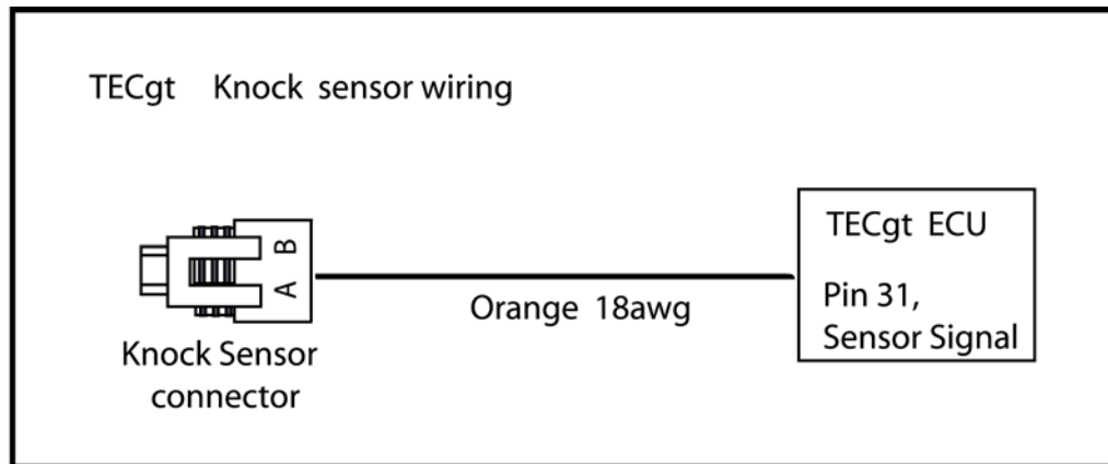
Fig G.7.1: Knock sensor wiring.
