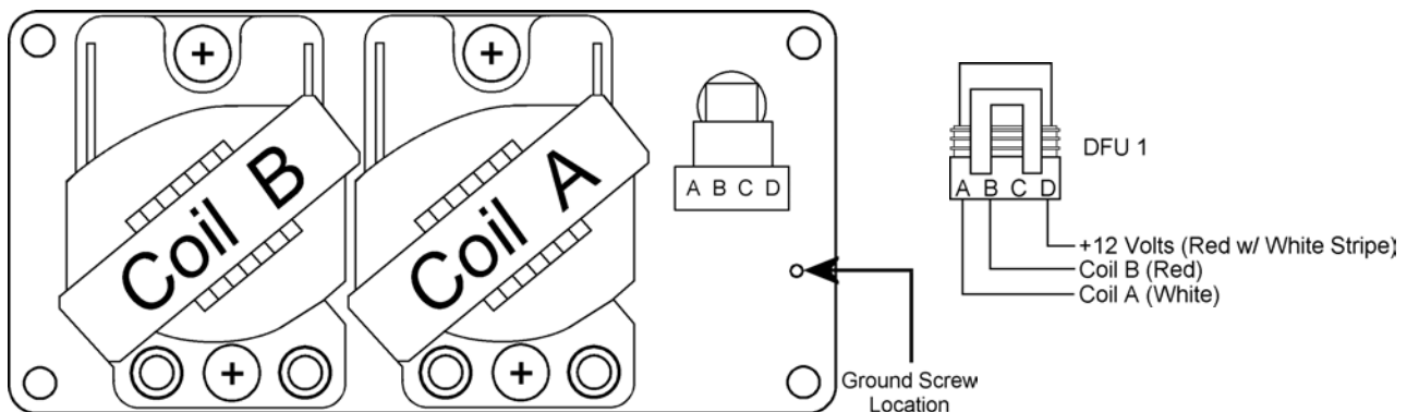
Figure C.2.2 : 4-Cyl DFU Setup
