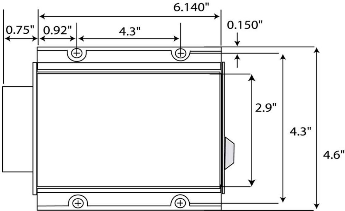
TECgt ECU Dimensions (bolt pattern is 4.3" x 4.3")
